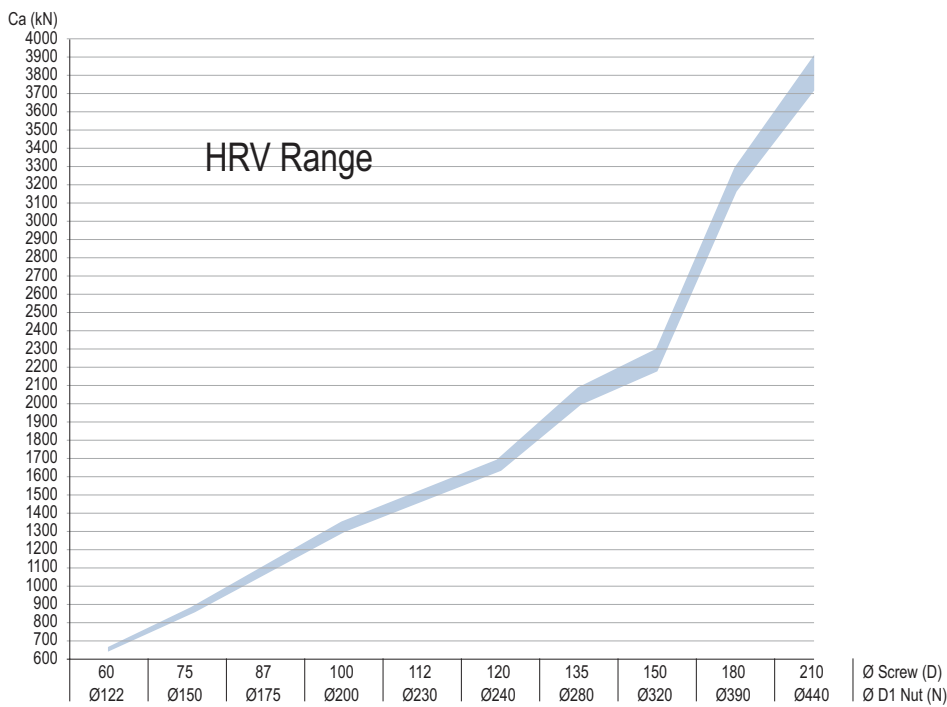
Dynamic capacities (Ca) diagram for roller screws as a function of the standard dimensions for standard HRV roller screws range
