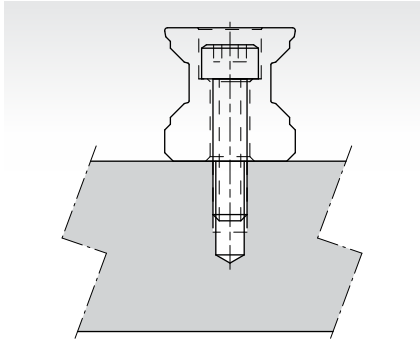
Counter bore (R type)
