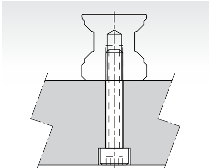
Tapped Hole (T type)
